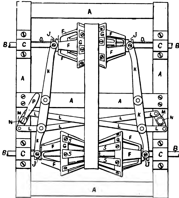
FIG. 348.—Diagram of a Variable Cone Pulley Transmission, by which the relative speeds of the driving shaft and counter shaft may be varied by changing the diameters of the driving and driven pulleys. In this figure, A is a frame on which are mounted the two shafts, B and B', turning in the bearings, C and C'. On each of these shafts is a feather, D, on which slide double cones, F, F, F, F. To the apex, J, of each of these cones, are attached fingers, S, S, S, S, which are screwed to the heads, G, G, G, G, as shown. A handle, P, pivoted at N, may be turned in either direction, actuating the levers, L, L, L, L and K, K, K, K; thus modifying the belted diameter of either pulley from that shown in the upper of the two to that shown in the lower one. Thus the speed ratios in the two may be varied to any desired point. The levers, K, K, K, K, by forked connections, actuate the cones, causing them to slide along the feathers, D, D, D, D, at the spools, J, J, J, J. The device shown in this illustration is the subject of an American patent; but similarly arranged and operated cone pulleys have been employed on the Foulliarion carriage and others.
